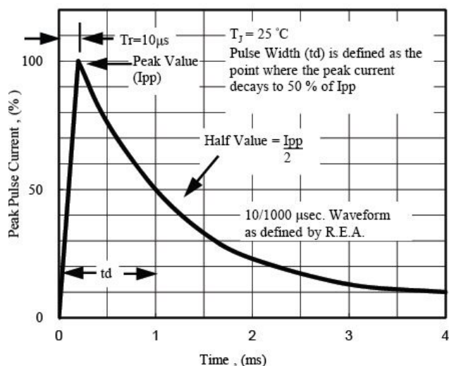
Fig. 5 - Pulse Waveform
